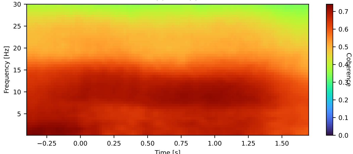
dPFC (4) - dPFC (6)
